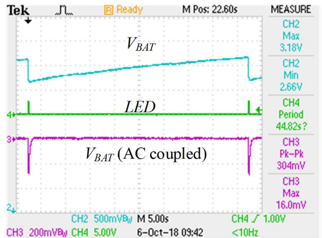
Fig. 20. Variation of the working voltages during long term operation.
